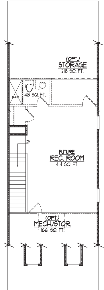
THIRD FLR./ ATTIC PLAN
