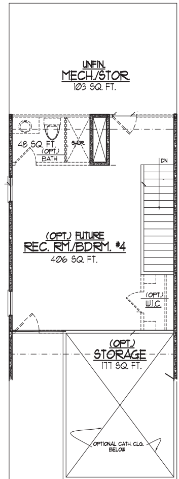
THIRD FLR./ ATTIC PLAN
